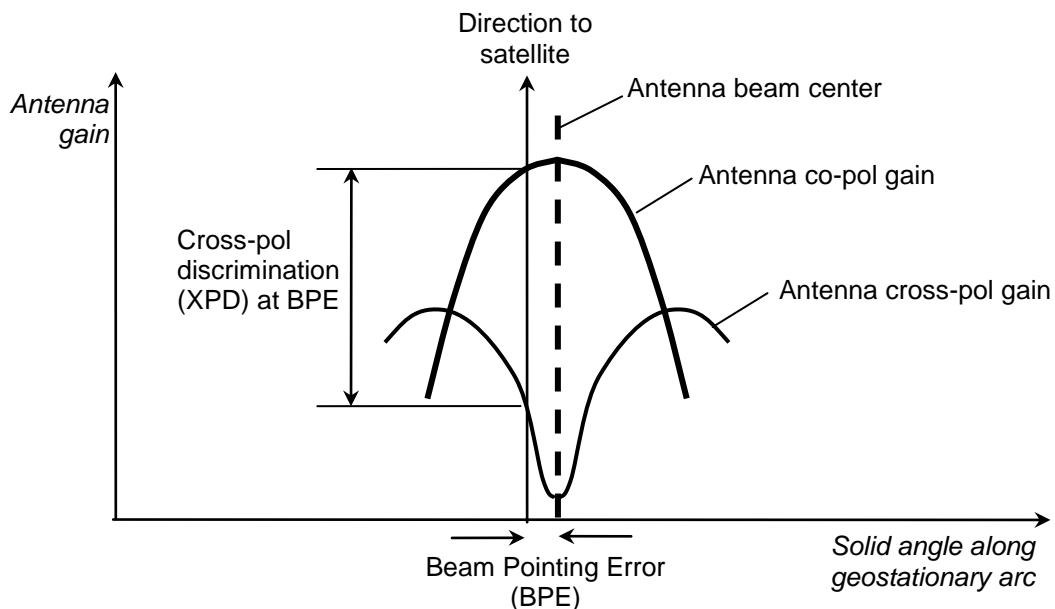
Figure 2. Cross-pol discrimination and BPE
