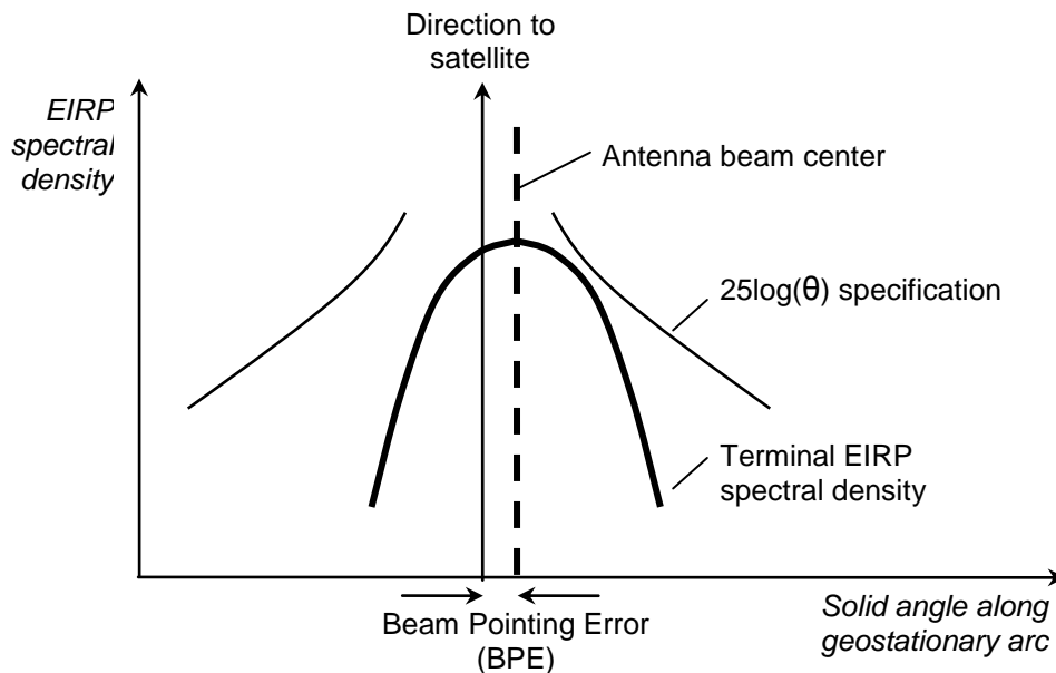
Figure 1. Off-axis EIRP spectral density and BPE
